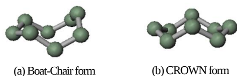
Figure 3 Semi-empirical optimized geometries of cyclooctane.
